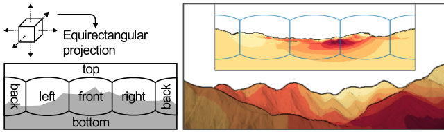
Figure 3: Visibility panorama. The diagram illustrates the generation of the 360° overview via environment mapping and equirectangular projection (left). Activating the widget allows for inspecting relevant information in the immediate vicinity of the viewer (right).
