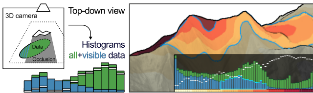
Figure 5: Visibility histogram. The diagram summarizes the computation of the histograms (left). The widget shows the relationship between distributions of visible values (blue) and all values (green) inside the current view (right). A white marker per bin indicates the percentage of occlusion in the respective value intervals. A narrow color legend helps associating bins and data values (bottom). When selecting one or multiple bins the respective data values are highlighted in the 3D view.
