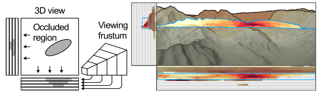
Figure 4: Visibility bands. The diagram illustrates how occluded information inside the camera’s viewing frustum is successively projected onto both image axes (left). The widget visualizes the projected information via horizontal and vertical bands, each with 16 layers ordered by distance to the viewer (right). When selecting one or multiple layers related occluded data are shown in the 3D view.
