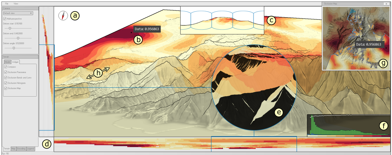
Figure 1: Schematic overview of our visualization tool. The main 3D view shows color-coded data embedded in terrain (middle). The user interface supports loading different terrain models, adjusting the visual encoding, and switching between multiple data attributes (left). An interface skin with light colors helps to focus on the main visualization. Our tool integrates four widgets and a rich set of coordinated interactions for showing hidden information and details on-demand: (a) compass, (b) tooltips, (c) panorama view, (d) bands view, (e) interactive lens, (f) histogram view, (g) 2D overview map, and (h) multi-perspective 3D view.
