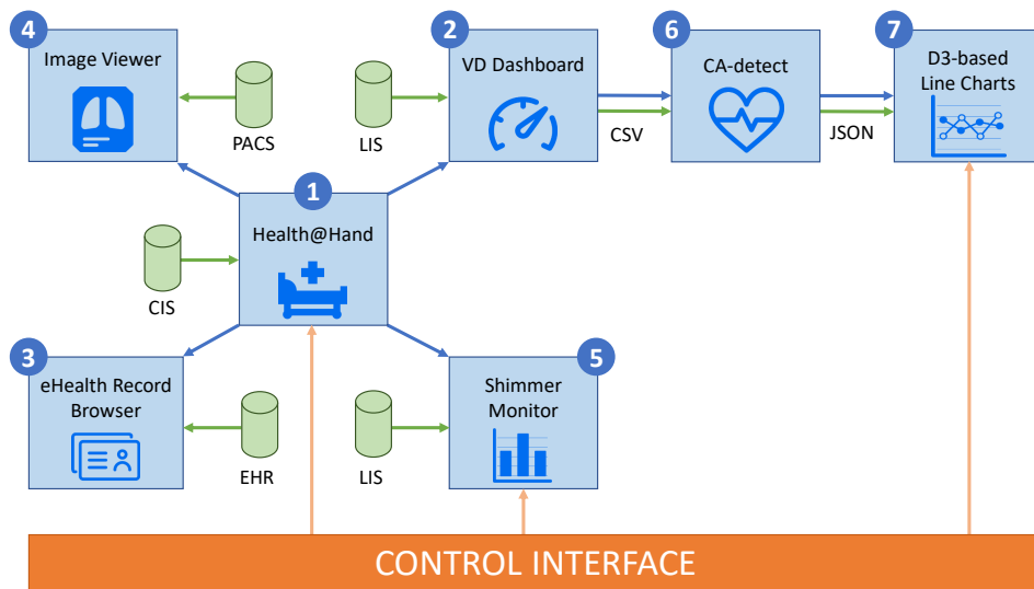
Figure 6: Combined view of a coordination model and the respective UI setup for a medical analysis scenario to detect cardiovascular symptoms and anomalies within a patient’s past and present clinical data utilizing multiple interlinked VA tools. The workflow is denoted with blue arrows, the data flow with green arrows, and the control flow with orange arrows.
