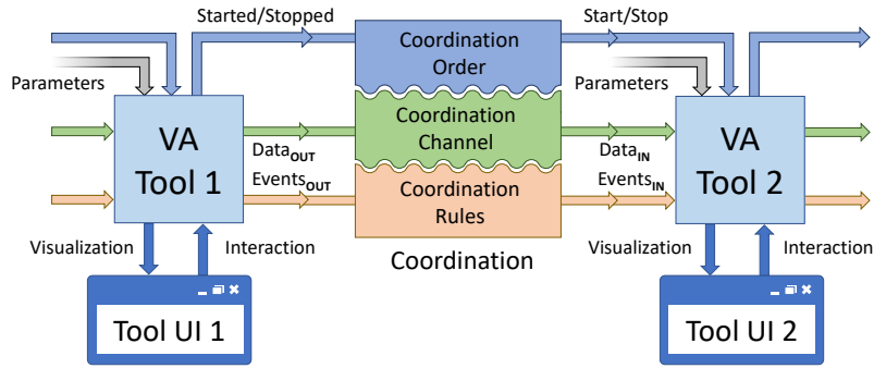
Figure 1: Conceptual abstraction of lightweight coordination between two VA tools. The coordination order models any temporal dependency between two tools (i.e., their subsequent or concurrent use). The coordination channels capture ways to exchange data between tools, including any necessary data transformations along the way. The coordination rules describe automated syncing features between tools as action/reaction pairs.
