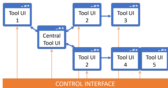
Figure 5: The control interface that serves as a global parametrization facility and for displaying process information. In this context VA tools can be utilized as a combination of single (UI 1 and UI 3), pair-wise (UI 4 and UI 5), and multiple (UI 2) references from a central hub application (Central UI).
